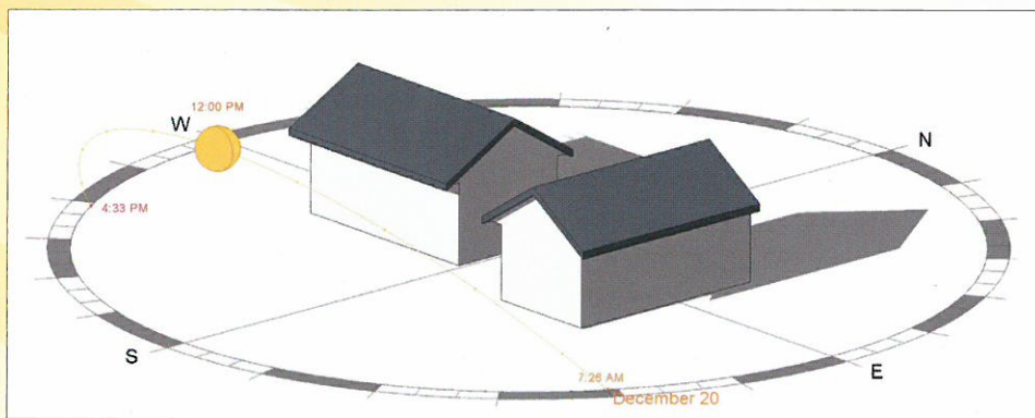
Figure 1: Solar exposure in the wintertime along south-facing walls. An east-west orientation provides the maximum opportunity for solar gain and solar heat penetration into the house.
